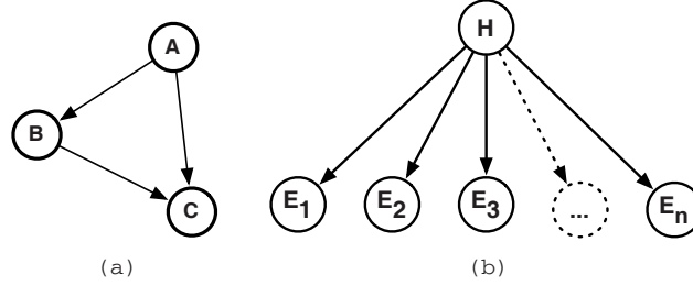
Figure 3. (a) is a simple Bayesian network. (b) is a naive Bayesian network.
